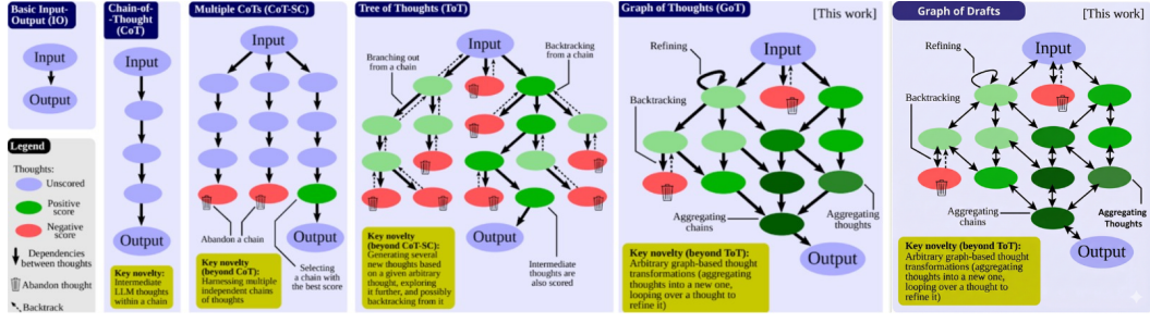
Fig. 1. Comparison of the GoD framework with existing approaches
