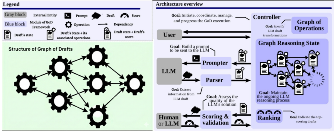
Fig. 3. System architecture of the GoD framework
